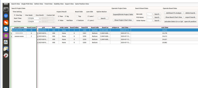
Inspection Statistics
