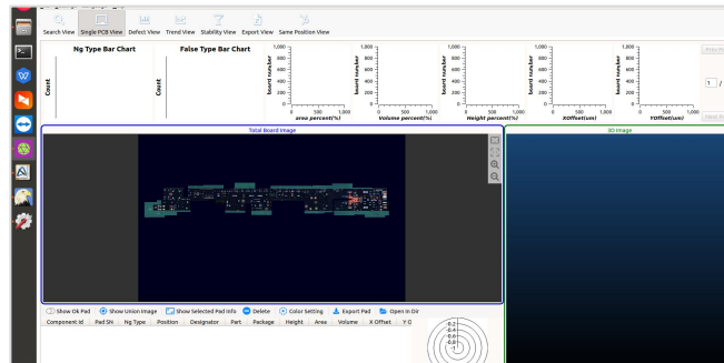
Defect Statistics
