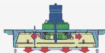
Heating Module
