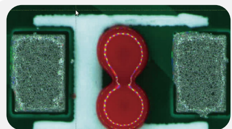
Red glue and solder paste imaging
