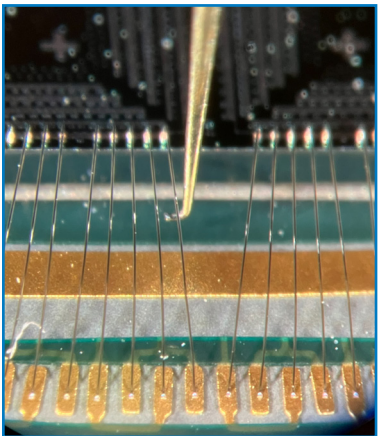
Wire pull Testing
