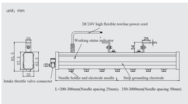
Ion bar size drawing
