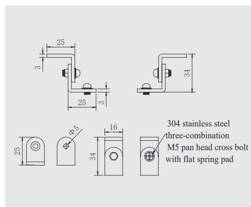
Mounting bracket size drawing
